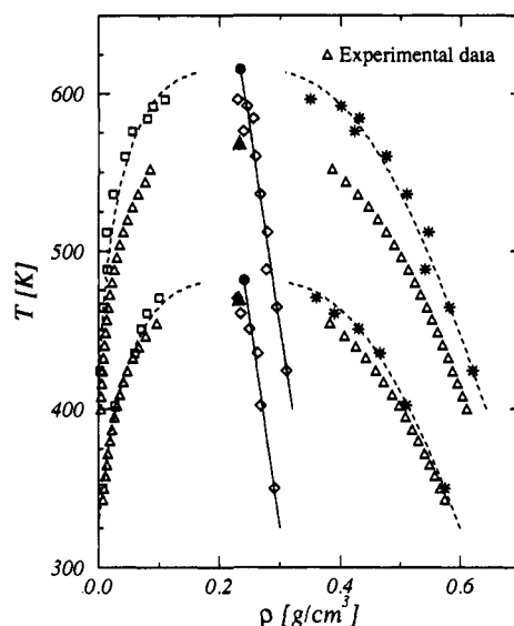
Figure 1. Vapor-liquid equilibria of pentane (lower curves) and octane (upper curves). \Delta are the experimental data and the \bullet is the experimental critical point. 19 \square , * are the vapor and liquid densities as obtained from our simulations. \diamond is the average of the liquid and vapor density. The solid lines are the fits to the scaling law and the rectilinear law. \bullet is the estimate of the critical point as obtained from these fits.
